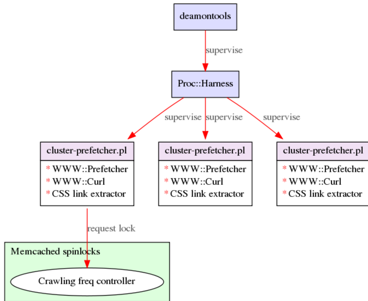
Prefetcher Internals
