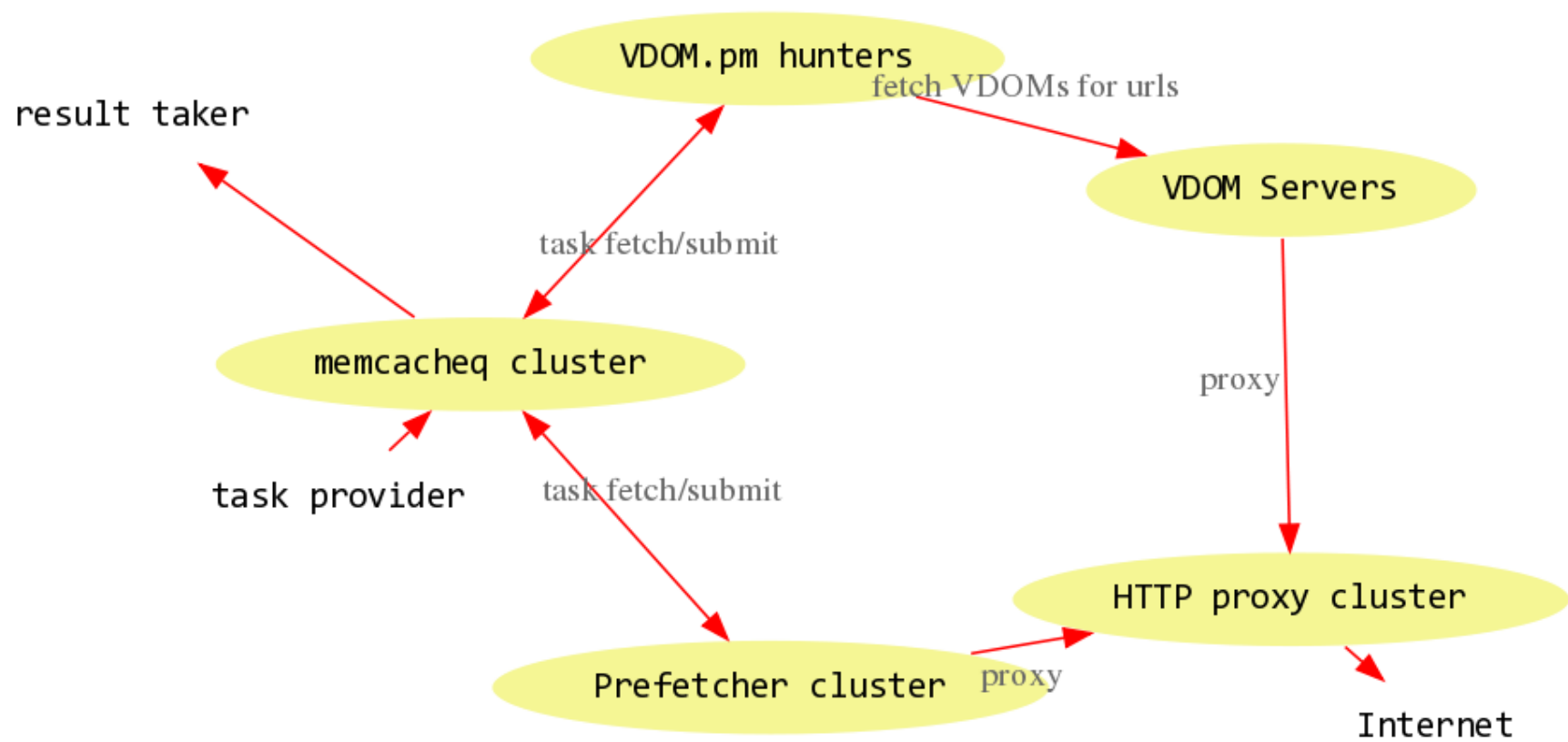
Architecture Diagram for our vdom-webkit Cluster
