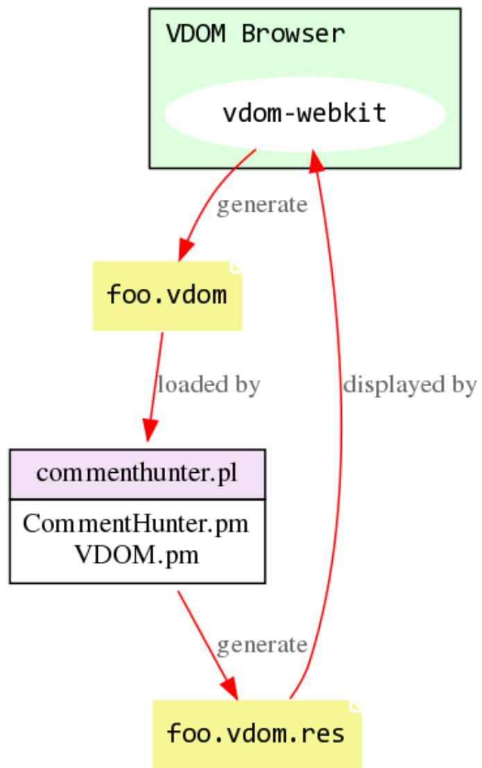
Interaction between VDOM Browser & VDOM.pm scripts
