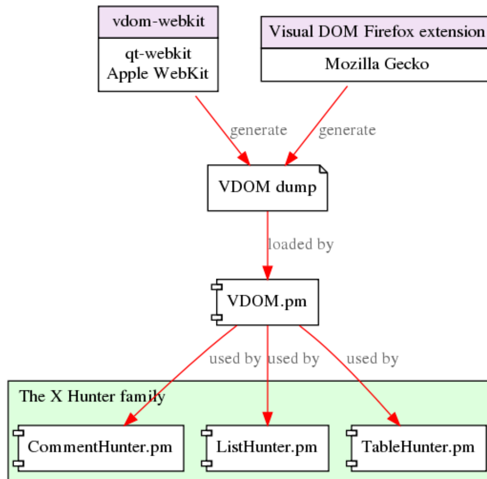
VDOM Data Flow
